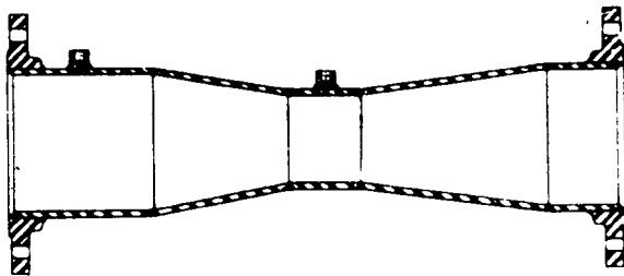
Flanged
