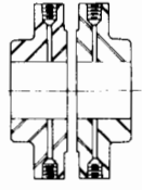
Slip On
